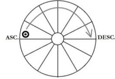
Diurnal Sect
