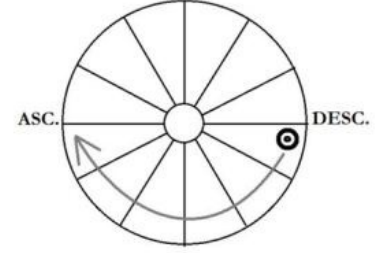
Nocturnal Sect
