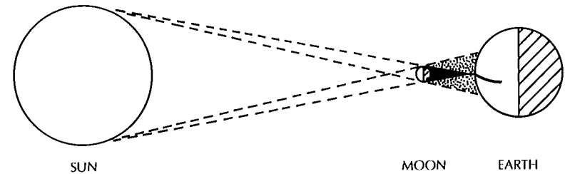
Total solar eclipse. The dark shadow is the umbra of total eclipse and the shaded area is the penumbra of partial eclipse. The dark line is the area on Earth where the total eclipse is visible.
